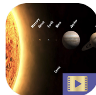
Solar System
